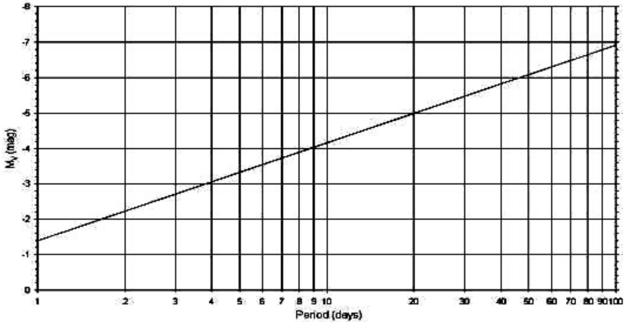
Period-Luminosity Relation
