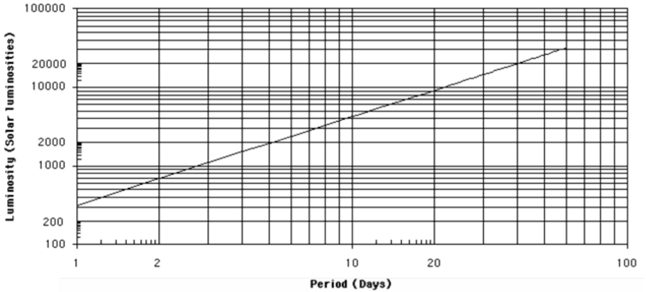
Period-Luminosity Relation from Hipparcos
