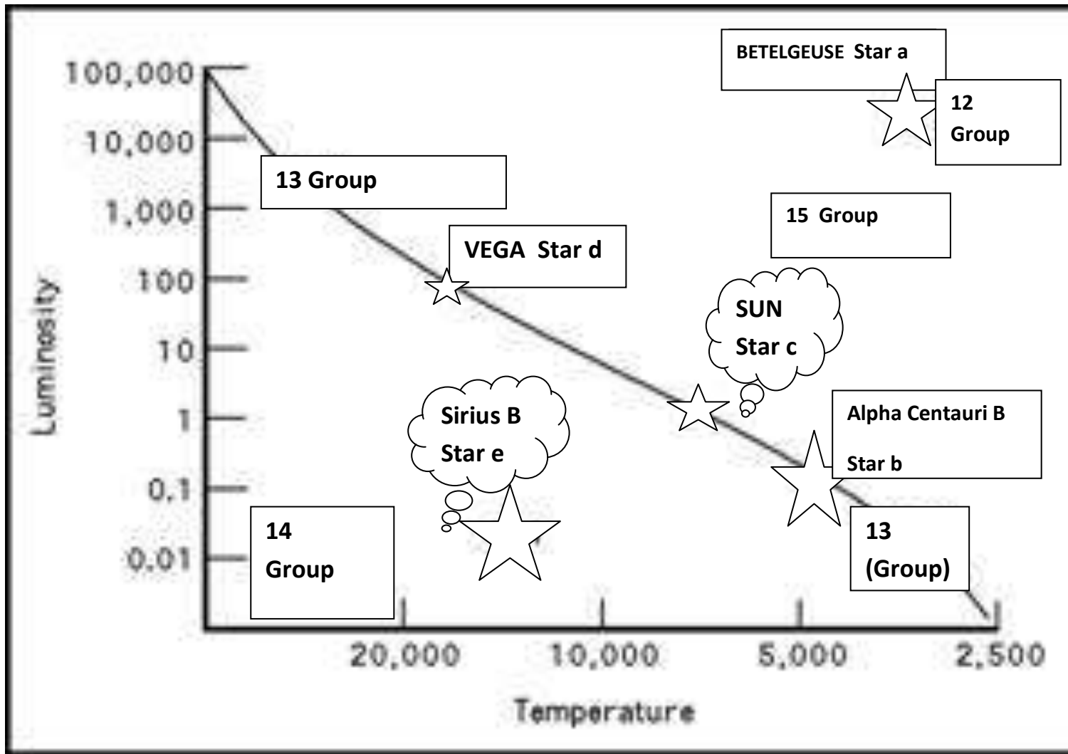
HR Diagram for Part 2, Section A Questions 1-15
